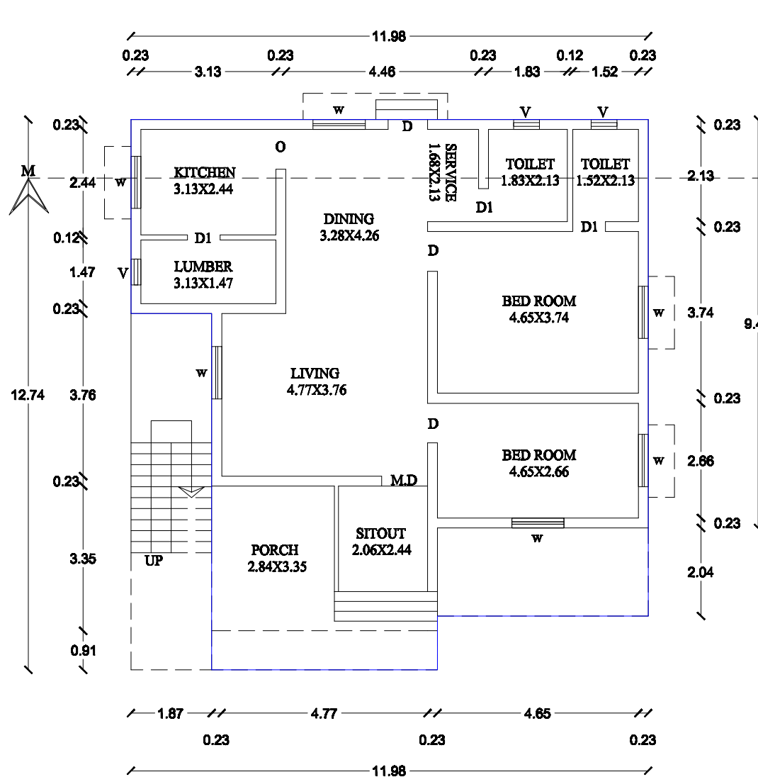
EXI - GROUND FLOOR PLAN
