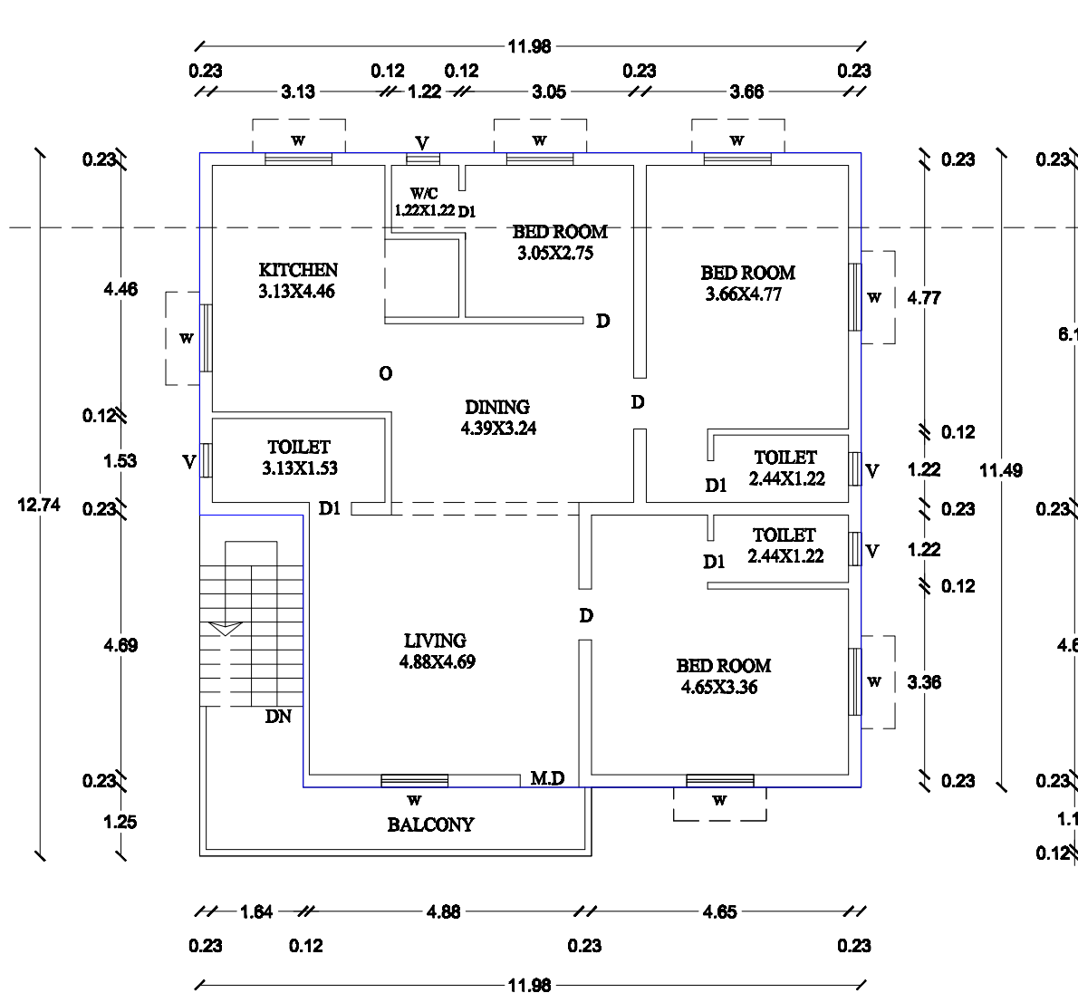
EXI - FIRST FLOOR PLAN
