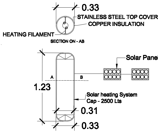
PLAN OF SOLAR WATER HEATING SYSTEM SCALE 1:50
