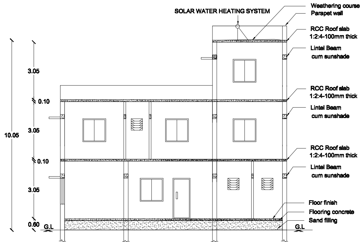
SECTION ON MK
