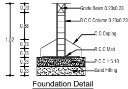
Foundation Detail
