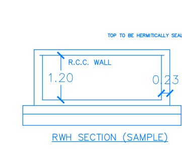
RWH_CAPACITY_L = 2000LTRS
