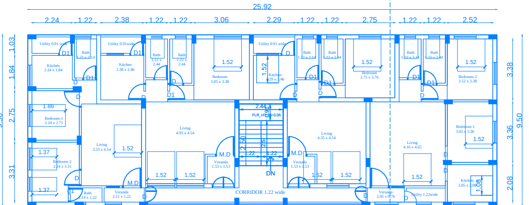
EXI.GROUND FLOOR PLAN
