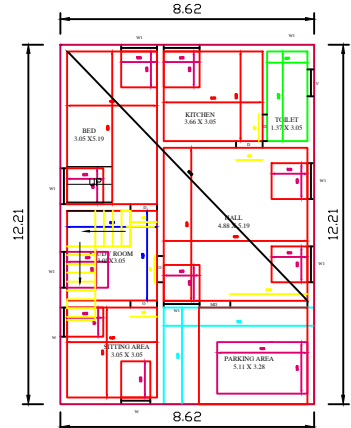
EXISTING GROUND FLOOR PLAN
