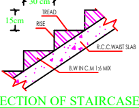
SECTION OF STAIRCASE
