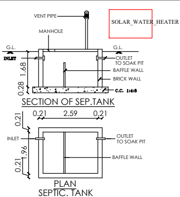
PLAN SEPTIC. TANK
