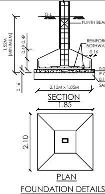
FOUNDATION DETAILS
