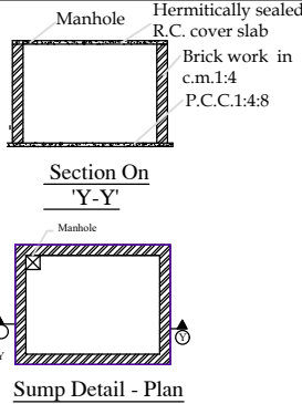
Sump Detail - Plan
