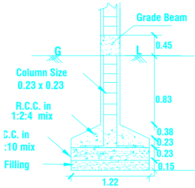
COLUMN DETAILS
