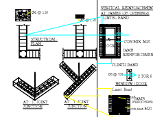
PRO. GROUND FLOOR PLAN DETAILS OF EARTHQUAKE :
