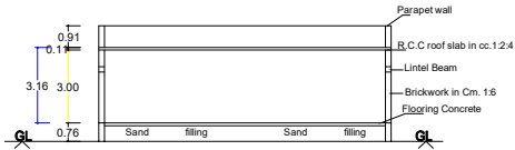
SECTION ON 'AB'
