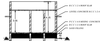
SECTION ON-"AB"
