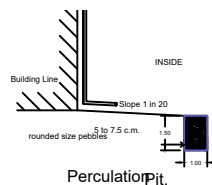
Percolation pit
