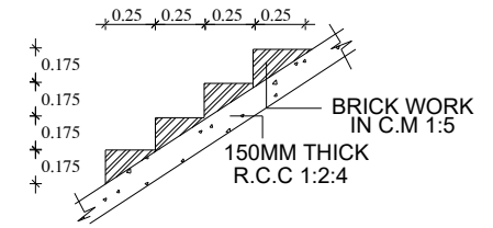
STAIRCASE DETAILS
