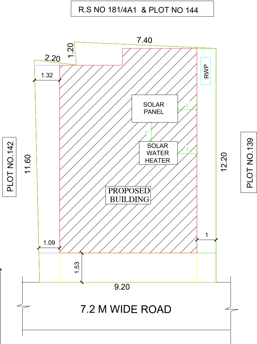
SITE PLAN
