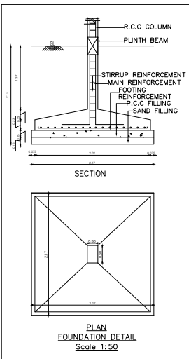
PLAN FOUNDATION DETAIL Scale: 1:50
