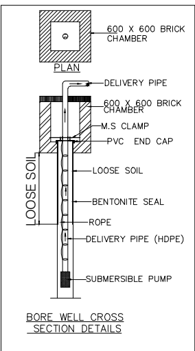
BORE WELL CROSS SECTION DETAILS
