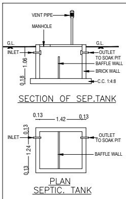
SECTION OF SEPT. TANK
