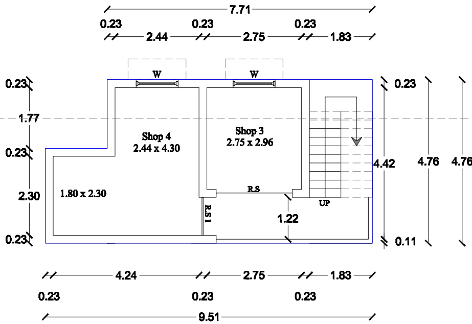
EXI - FIRST FLOOR PLAN
