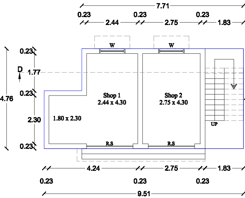
EXI - GROUND FLOOR PLAN
