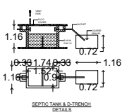
SEPTIC TANK & TRENCH DETAILS (NTS)
