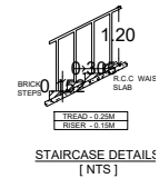
STAIRCASE DETAILS (NTS)
