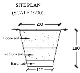
Trail pit details NOT TO SCALE
