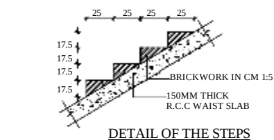
DETAIL OF THE STEPS SCALE 1:100
