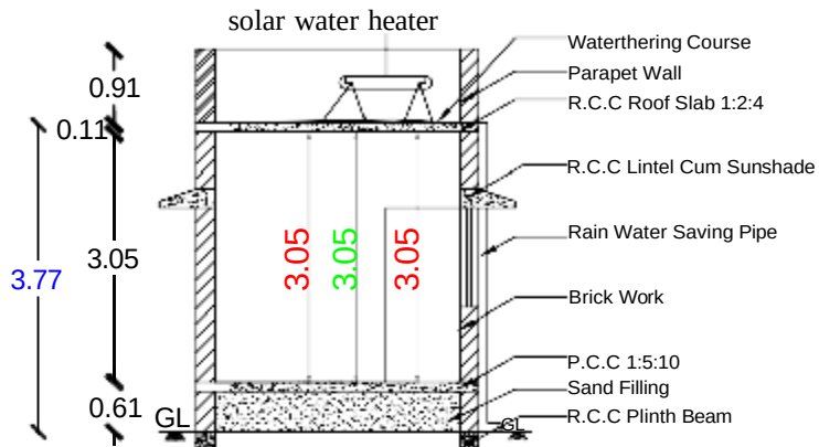
SECTION AB
