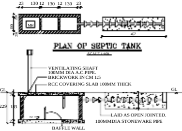
SECTION OF SEPTIC TANK SCALE 1:100
