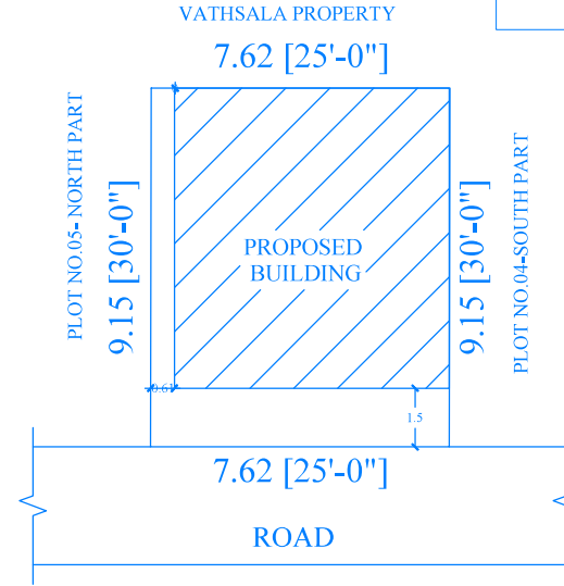
SITE PLAN
