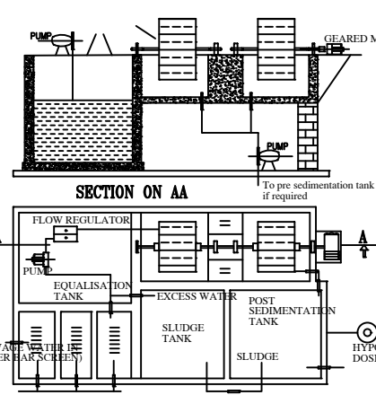
SEWAGE TREATMENT PLANT DETAILS
