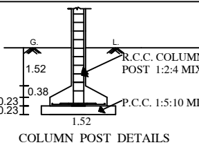
SEWAGE TREATMENT PLANT DETAILS
