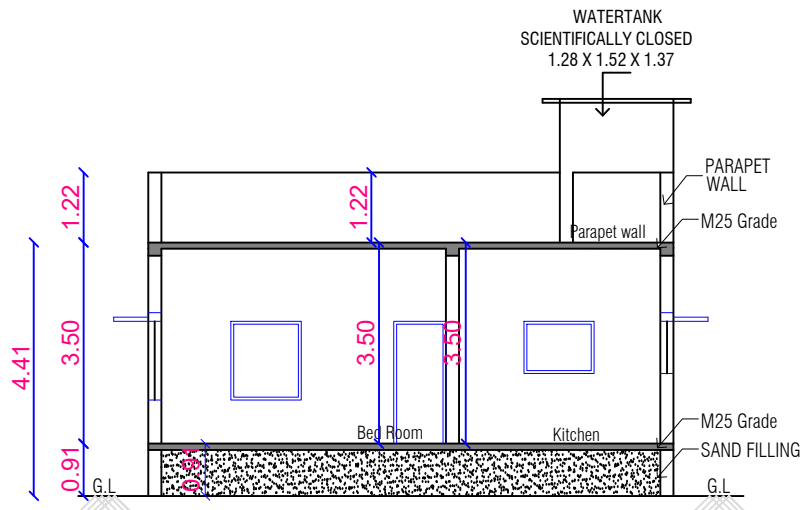
SECTION - AA (PROPOSED)
