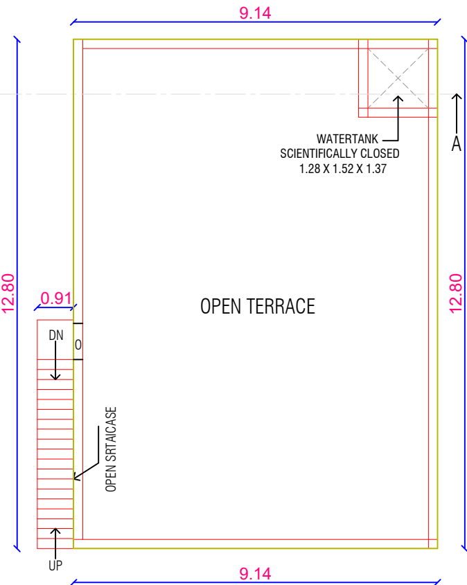
TERRACE FLOOR PLAN (PROPOSED)
