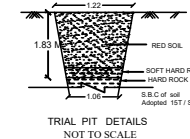
TRIAL PIT DETAILS NOT TO SCALE
