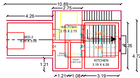
PRO-FIRST FLOOR PLAN
