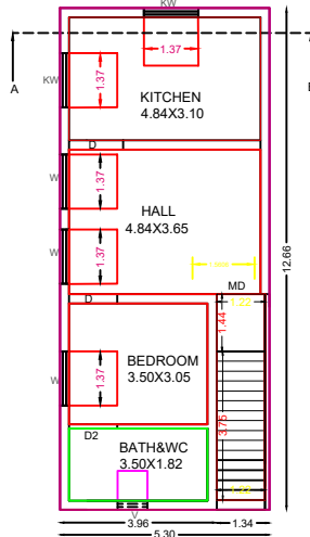
PRO.FIRST FLOOR PLAN
