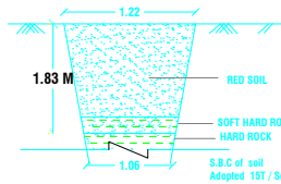
TRIAL PIT DETAILS NOT TO SCALE
