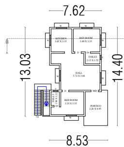
PRO.GROUND FLOOR PLAN
