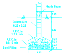
COLUMN DETAILS NOT TO SCALE
