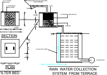
RAIN WATER COLLECTION SYSTEM FROM TERRACE
