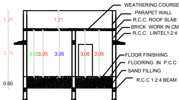
SECTION
