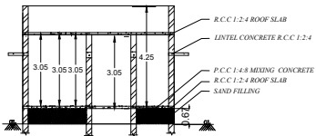
SECTION ON-AB
