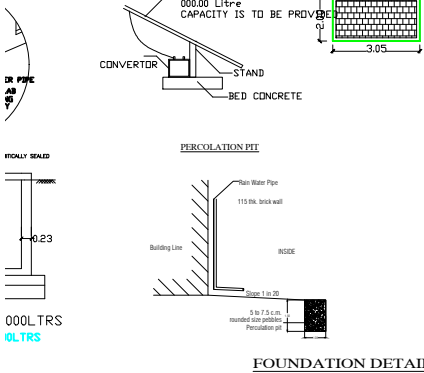
VESTING: SOLAR SYSTEM LONGITUDINAL SECTION
