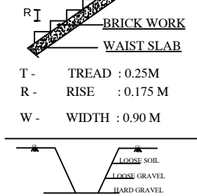
STAIRCASE DETAILS (NOT TO SCALE)
