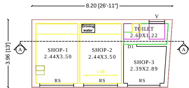
PRO.GROUND FLOOR PLAN
