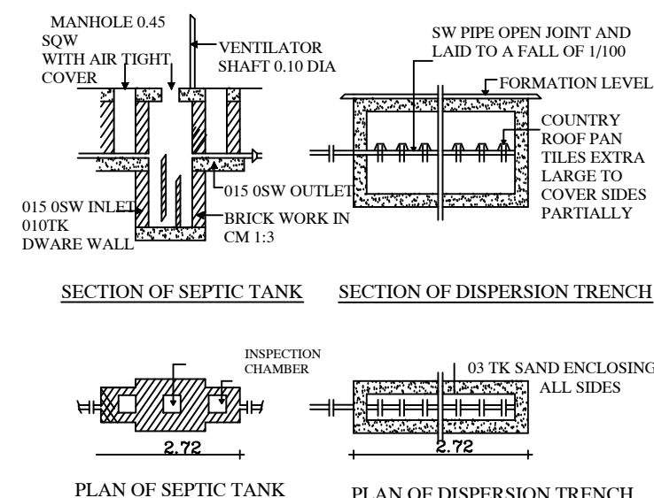
PLAN OF SEPTIC TANK
