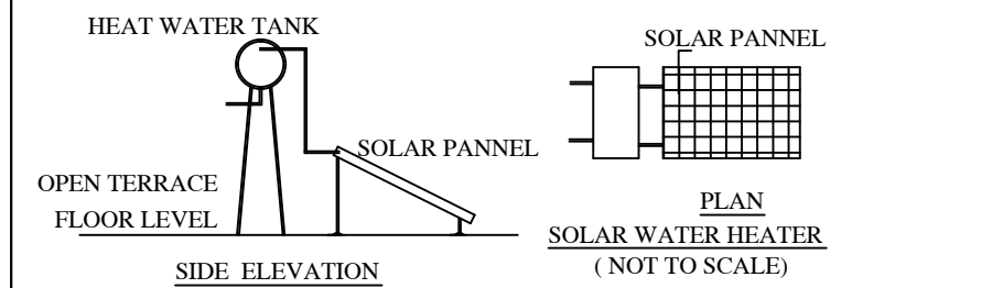
SIDE ELEVATION
