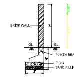
COMPOUND WALL DETAIL
