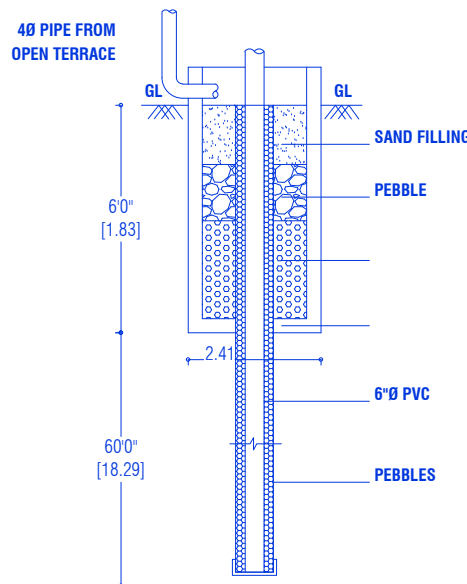
Section of Rain water Harvesting (from open terraced)
