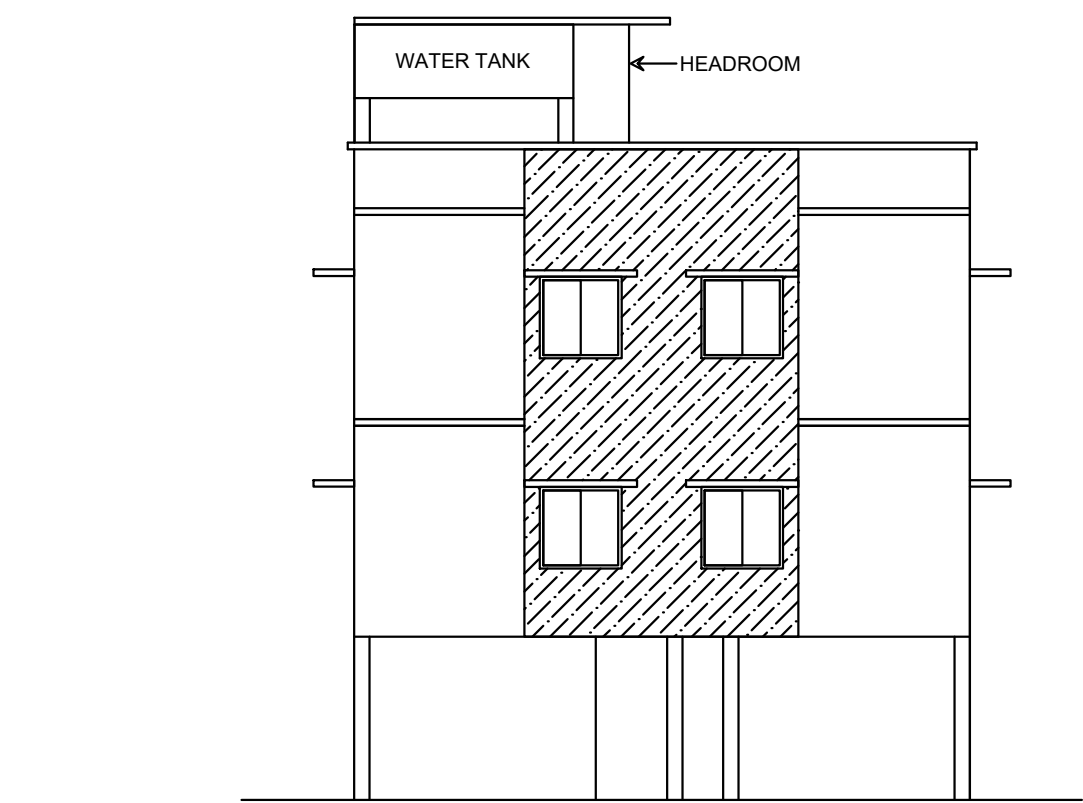
FRONT ELEVATION
