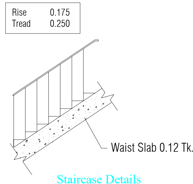
Staircase Details
