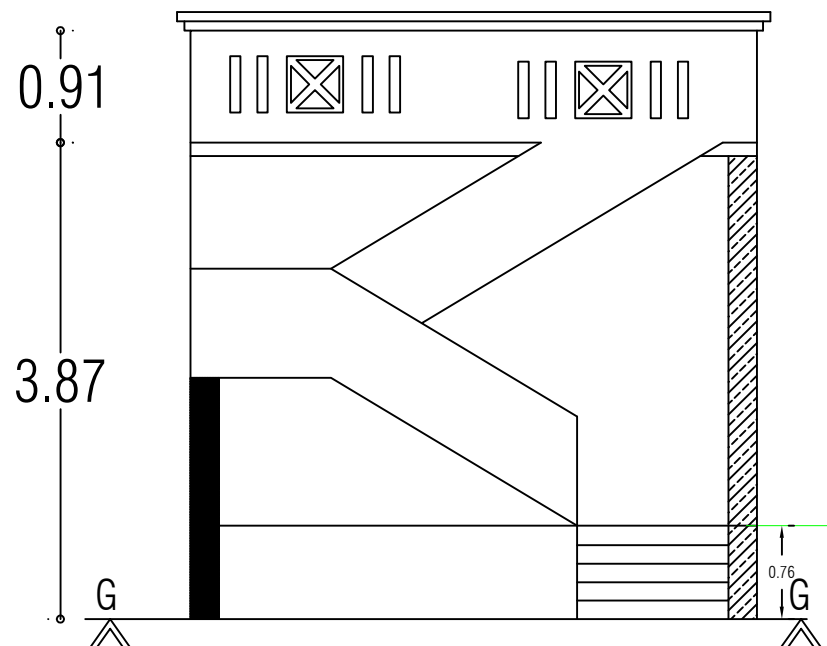
FRONT ELEVATION
