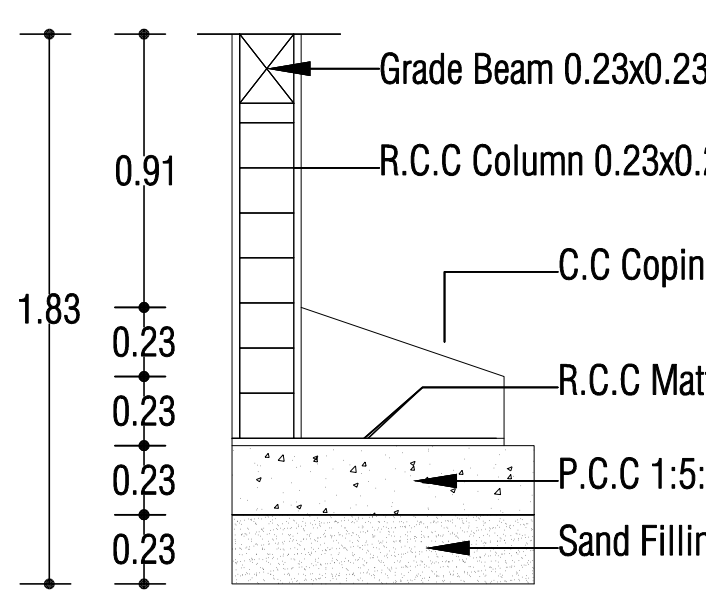
Foundation Details
