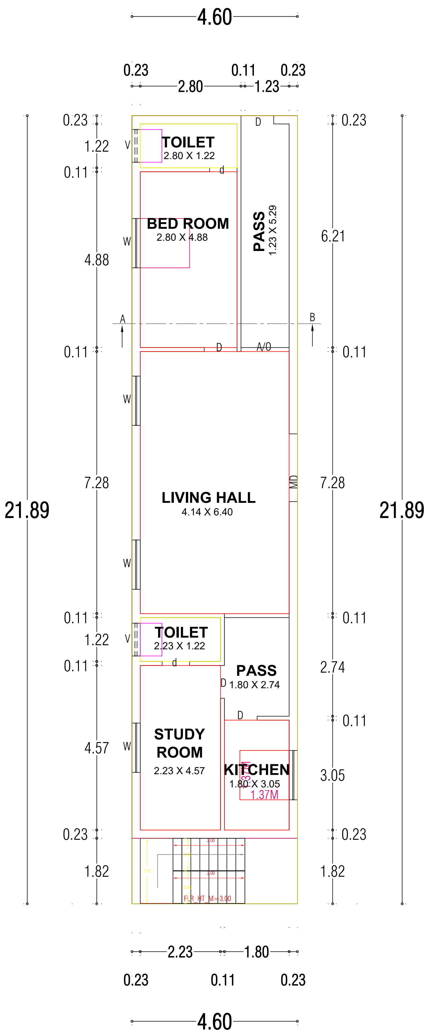
PRO GROUND FLOOR PLAN
