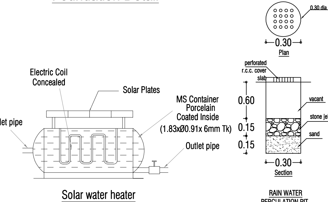
Solar water heater
