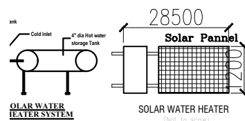
SIDE ELEVATION (Not to scale)
