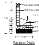
Foundation Details
