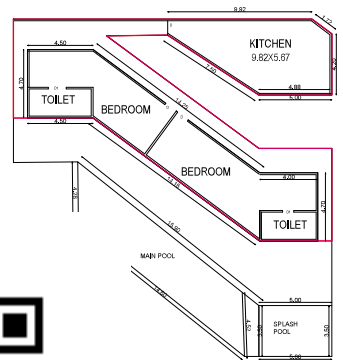
GROUND FLOOR PLAN BLOCK-1
