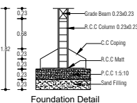
Foundation Detail
