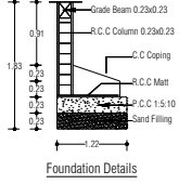
Foundation Details
