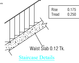
Staircase Details
