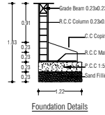
Foundation Details
