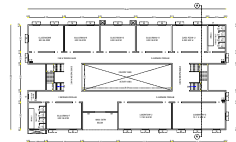
PROPOSED FIRST FLOOR
