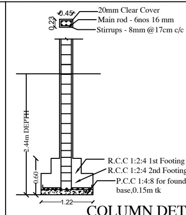
COLUMN DETAILS
