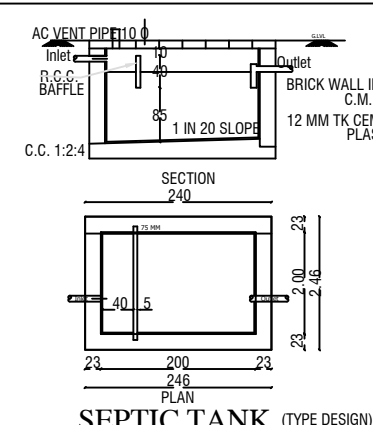
SEPTIC TANK (TYPE DESIGN)
