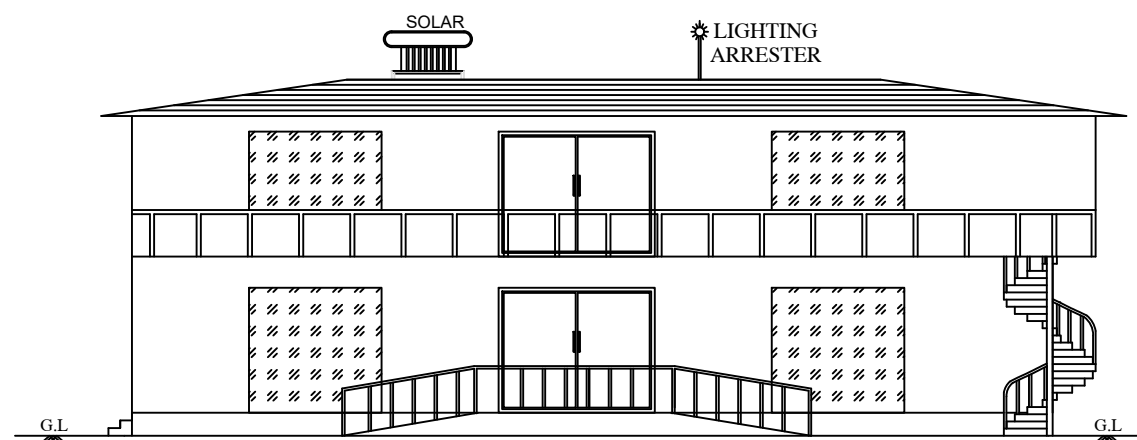
FRONT ELEVATION
