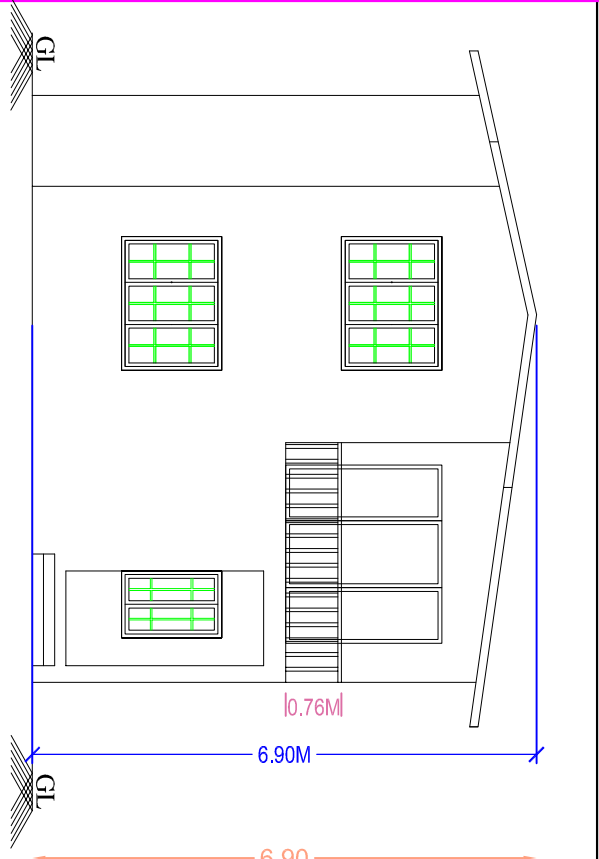
FRONT ELEVATION
