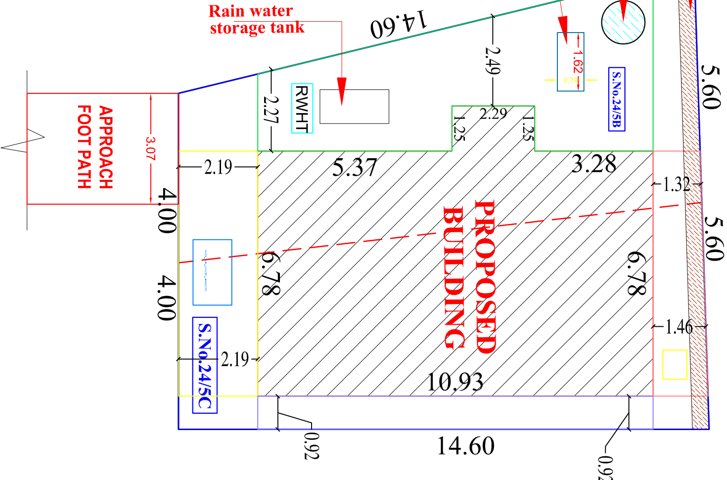
SITE PLAN
