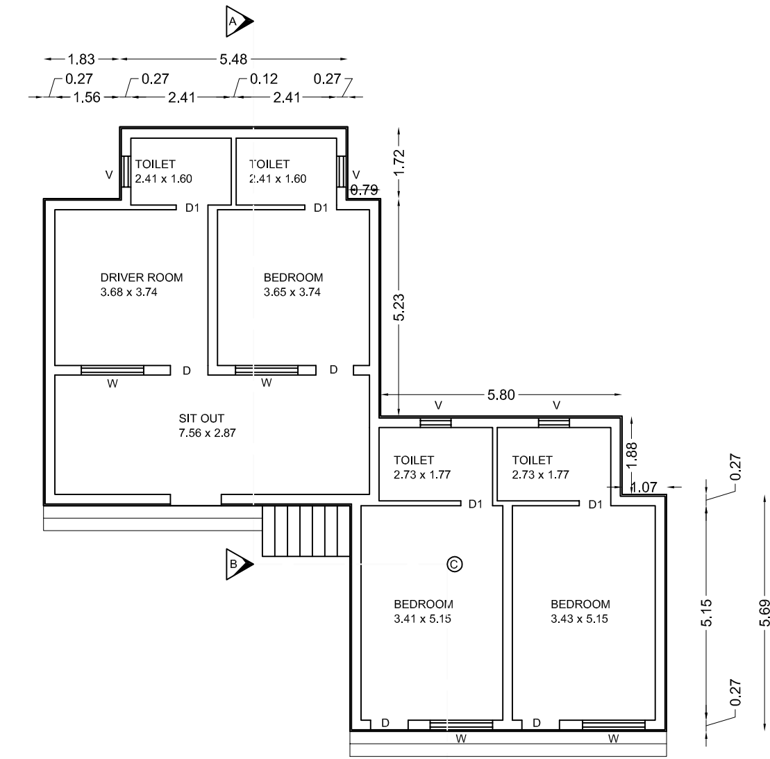
GROUND FLOOR
