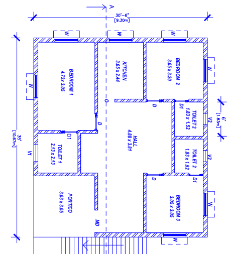
GROUND FLOOR PLAN AREA OF GROUND FLOOR - 881 Sq.M (1987.5 Sq.Ft)
