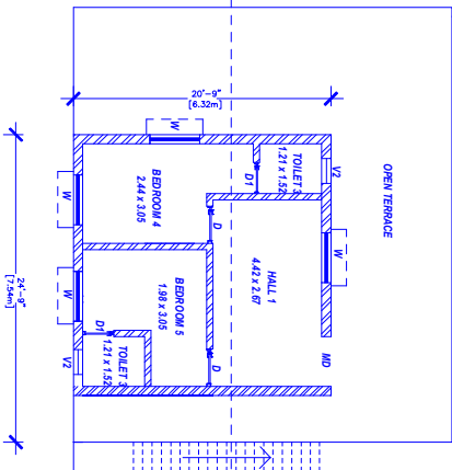
FIRST FLOOR PLAN AREA OF FIRST FLOOR - 401 Sq.M (832.5 Sq.Ft)
