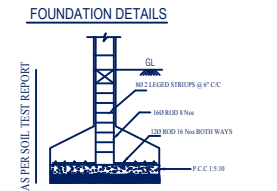
EARTH QUAKE SAFE DESIGN DETAILS
