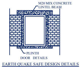
EARTH QUAKE SAFE DESIGN DETAILS
