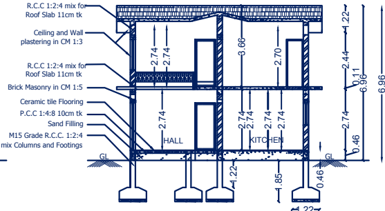
CROSS SECTION AT A-A
