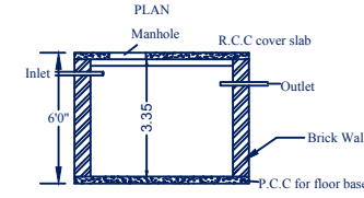
RAIN WATER HARVESTING TANK
