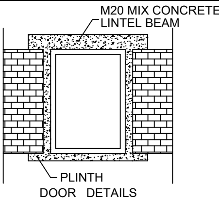
EARTH QUAKE SAFE DESIGN DETAILS
