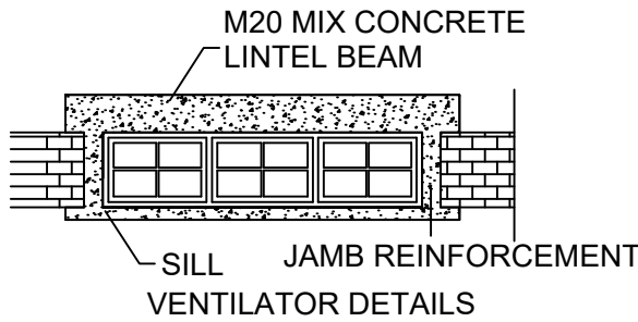
EARTH QUAKE SAFE DESIGN DETAILS
