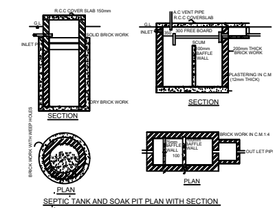
SEPTIC TANK AND SOAK PIT PLAN WITH SECTION
