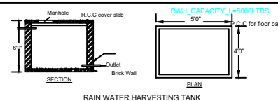
RAIN WATER HARVESTING TANK
