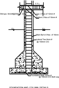
FOUNDATION AND COLUMN DETAILS
