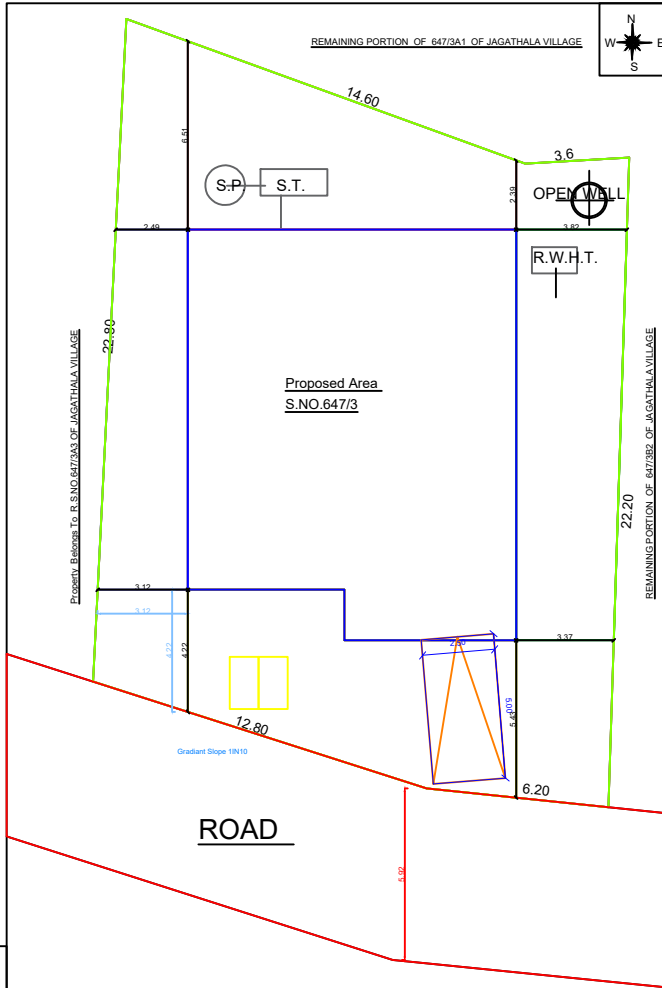
SITE PLAN
