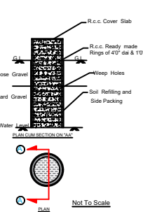
OPEN WELL DETAILS
