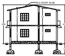
SECTION ON A - B
