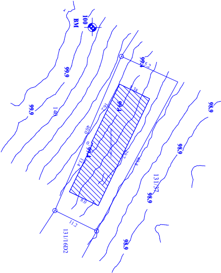
CONTOUR & TOPOGRAPHICAL PLAN
