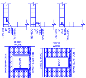
EARTHQUAKE SAFE DESIGN (NOT TO SCALE)
