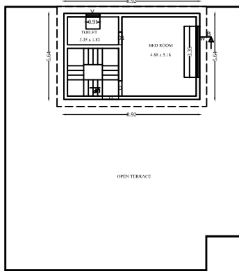
PROPOSED FIRST FLOOR PLAN
