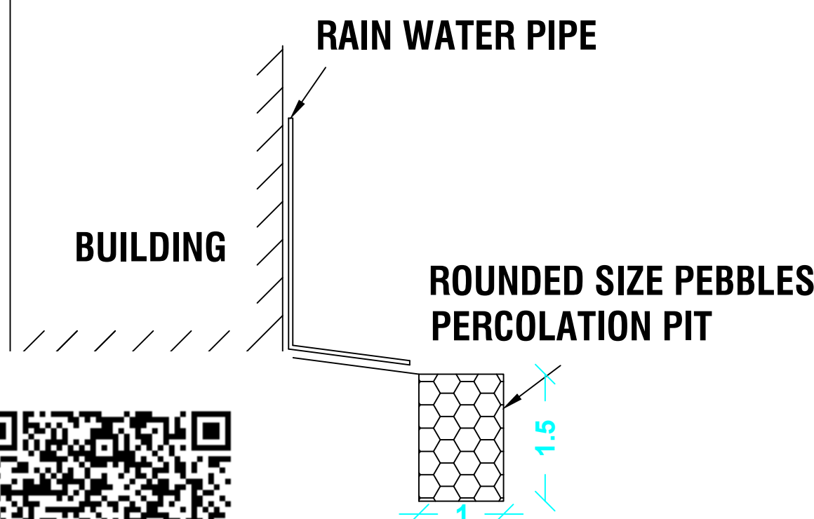
RAINWATER COLLECTING TANK
