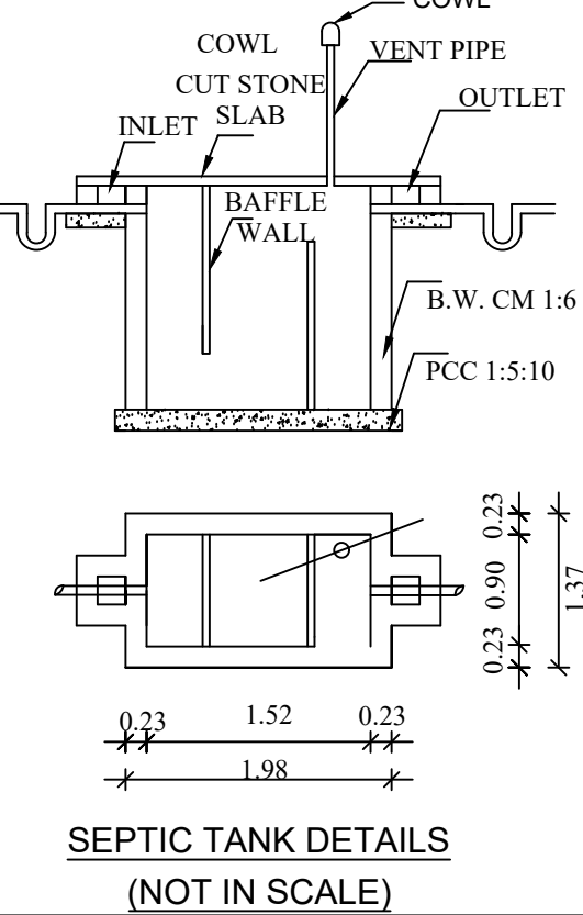
SEPTIC TANK DETAILS (NOT IN SCALE)
