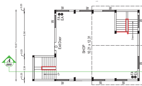
LOWER LEVEL FIRST FLOOR & UPPER LEVEL GROUND FLOOR
