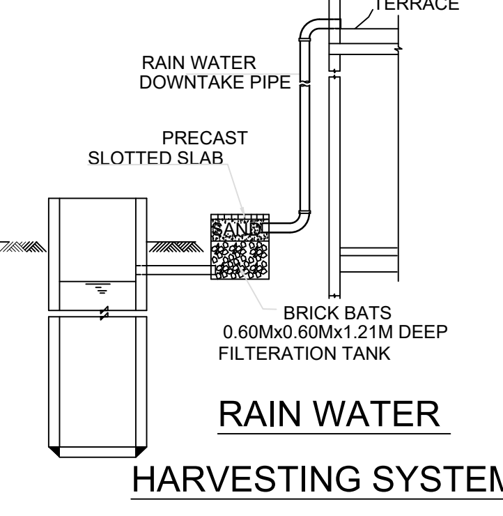
RAINWATER COLLECTION SUMP
