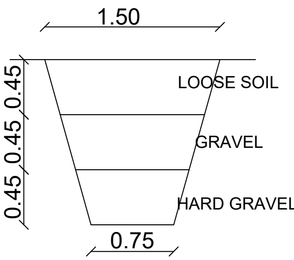
TRIAL PIT NOT TO SCALE
